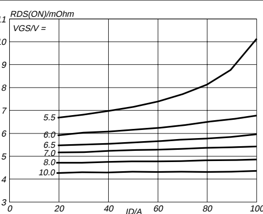
Fig.6. Typical on-state resistance, T_j = 25 °C. R_{DS(ON)} = f(I_D) ; parameter V_{GS}
